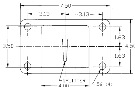
SUCTION FLANGE DETAIL
